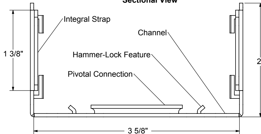
Sectional View
